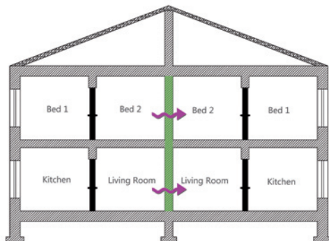
Sound test schedule for a development of 2 - 10 terraced houses.
